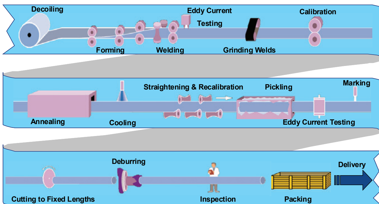
Fig. 1 Typical production route for inline strip welded tubes.
