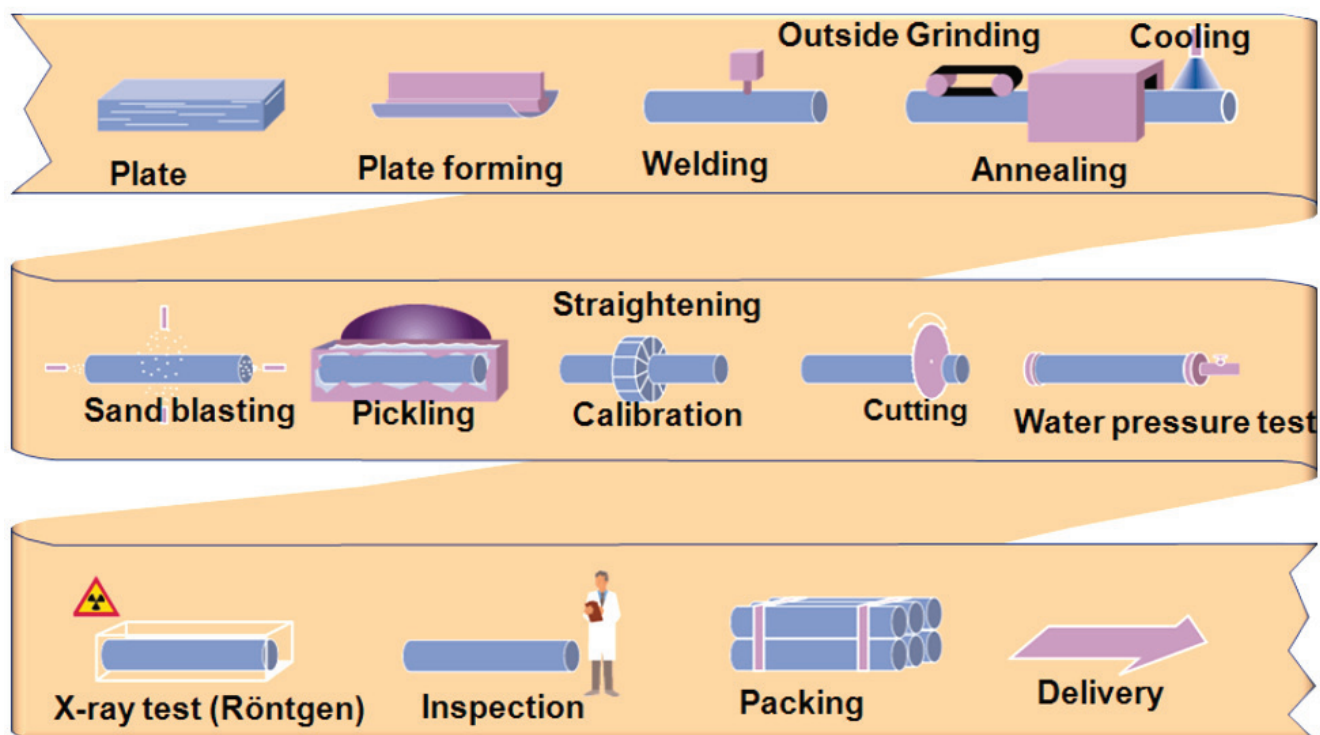
Fig. 2 Typical production route for heavy-walled pipes.
