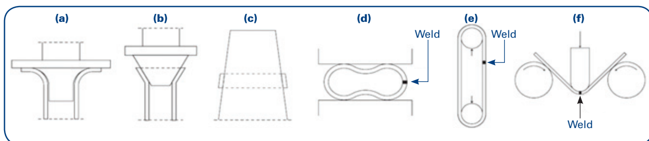
Fig. 5 Some examples of technological testing of tubes (a) flange test, (b) flaring test, (c) ring expansion test, (d) flattening test, (e) ring tensile test and (f) root bend test.
