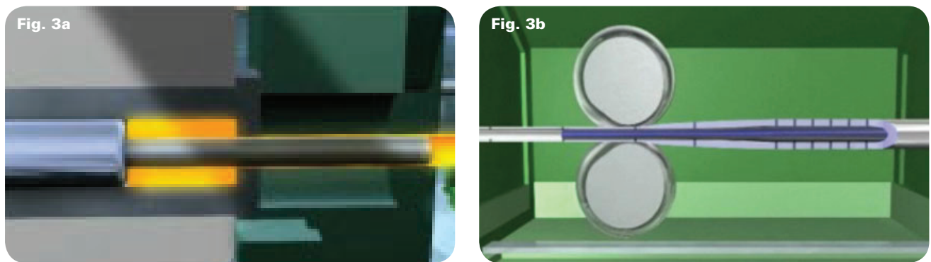
Fig. 3 (a) Extrusion of a seamless tube and (b) pilgering cold work [4].
