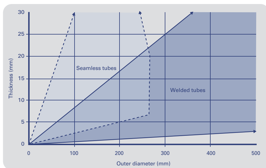
Fig. 4 Typical dimension areas for seamless and welded tubes and where these primarily overlap.
